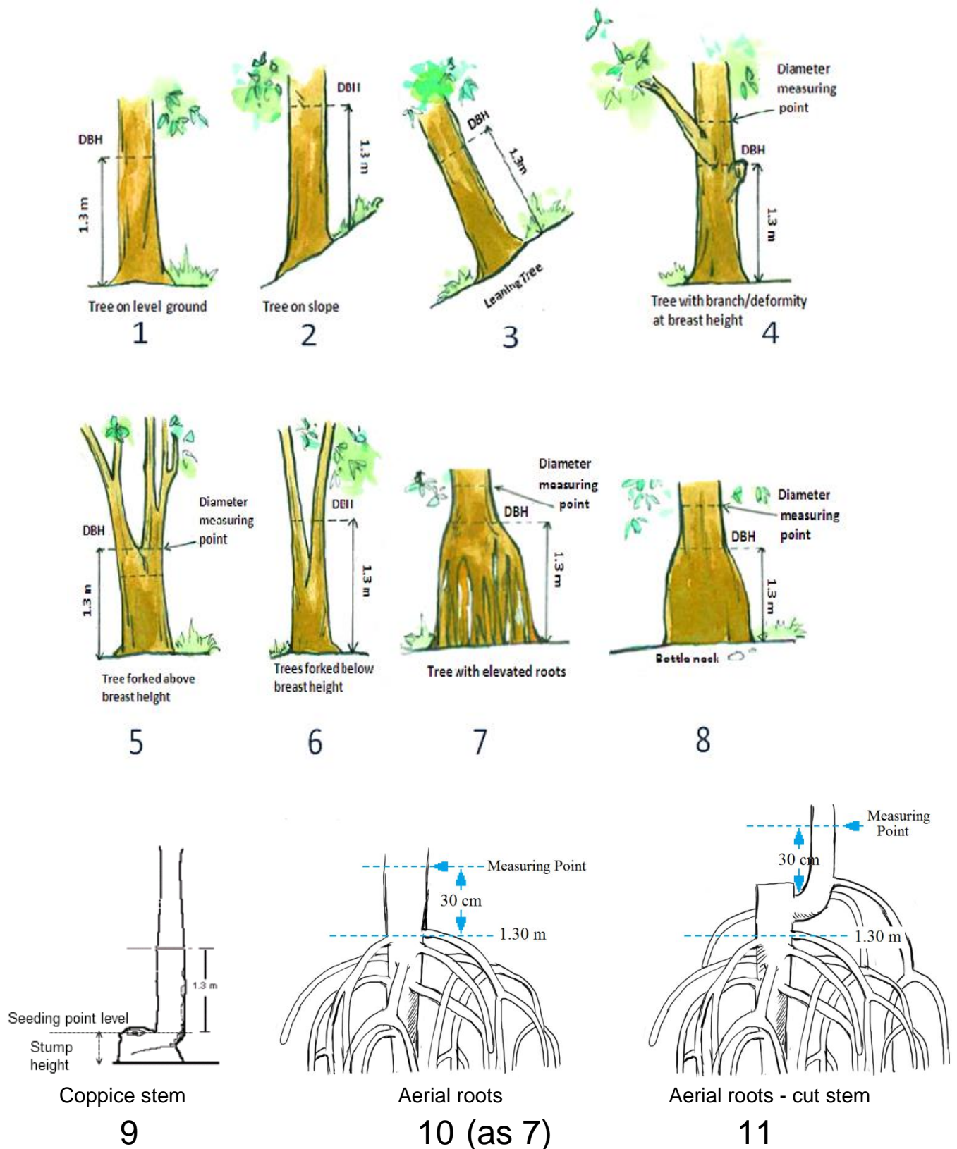
Figure 5. Measuring of breast height diameter (dbh)
