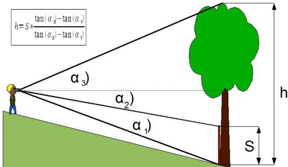
Figure 7. Tree height measurements
