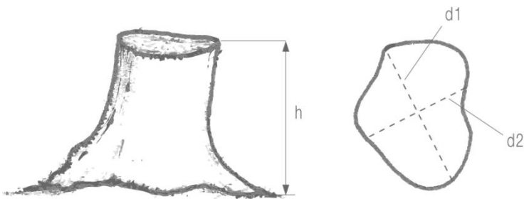
Figure 10. Measuring of stump diameter
