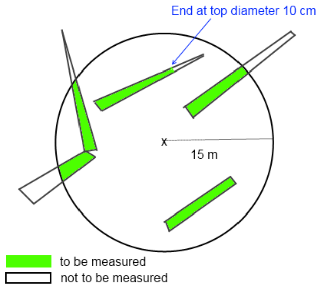
Figure 12. Selection of deadwood parts in the plot
