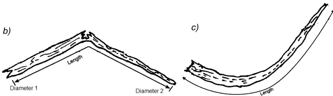
Figure 13. Deadwood measurements
